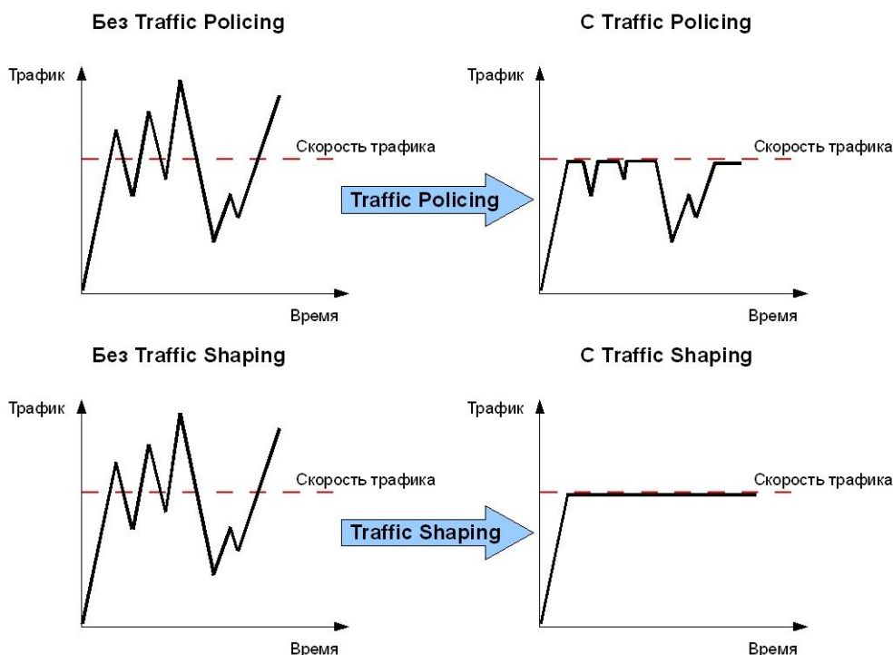
Рис. 6.8. Механизмы Traffic Policing и Traffic Shaping
